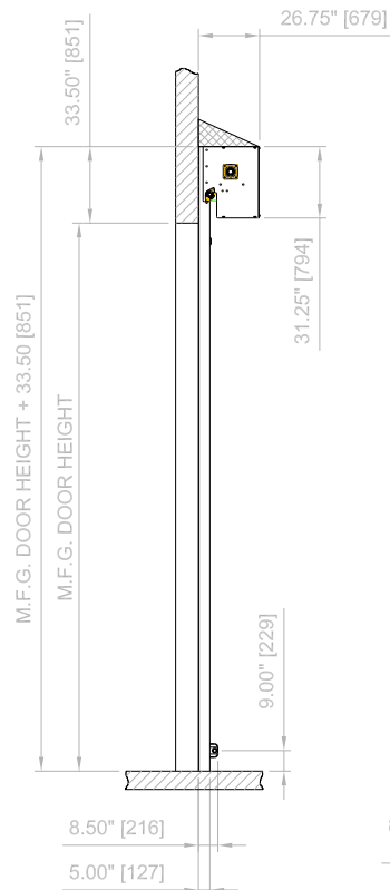
LEFT VIEW
