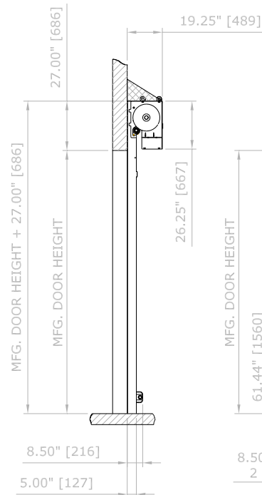
LEFT VIEW
