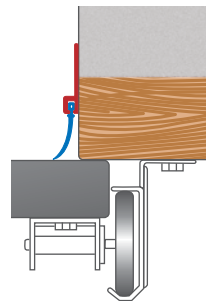
A0282-MI-W/B0772-00-W (3" STANDARD BRUSH SEAL, PG.5)
