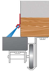
A0082-MI-W/B0768-00-W (1" STANDARD BRUSH SEAL, PG.5)
