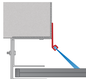
A0282-MI-W/B0772-00-W (3" STANDARD BRUSH SEAL, PG.5)
